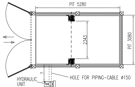
LOWER FLOOR-PLAN
